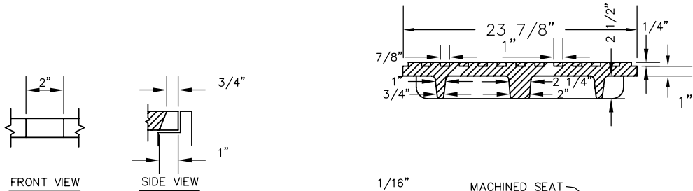
LIFTING NOTCH
